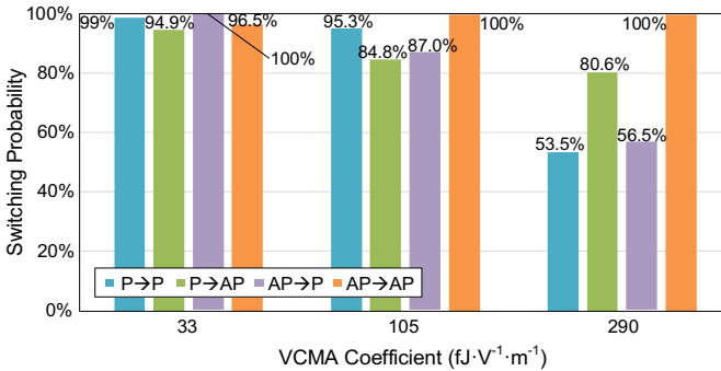
Fig. 13. Highest switching probability after optimizing V_E , V_{STT} , and pulse-width for different VCMA coefficients. Switching probabilities for all four directions are shown. Due to the unstable nature of VCMA, it is difficult to achieve switching probabilities required for practical memory applications.
