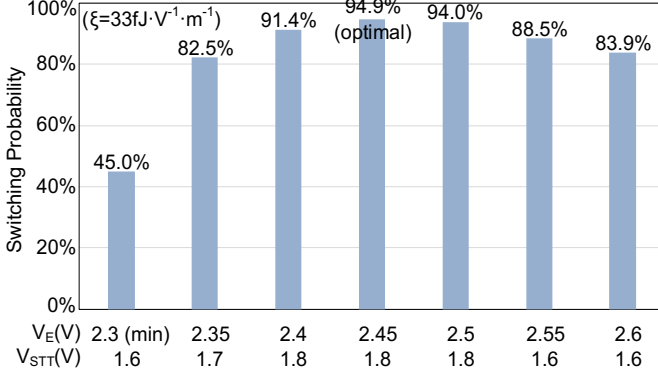
Fig. 12. Switching probability for different V_E voltages. V_E pulse-width and V_{STT} voltage were optimized for each V_E voltage.
