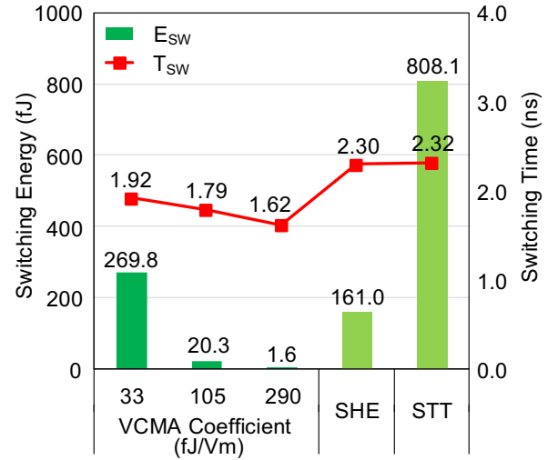
Fig. 6. Switching energy and switching time for VCMA, SHE and STT.
