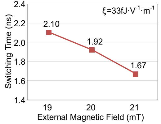
Fig. 10. Effect of external magnetic field on switching time.
