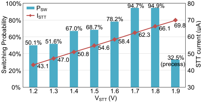
Fig. 11. Switching probability versus V_{STT} for V_E=2.45V .
