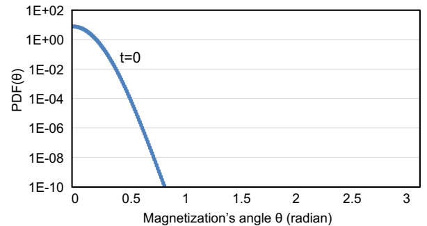
Fig. 2. Initial angle distribution, PDF(\theta)|_{t=0} , for TSF=45.7
