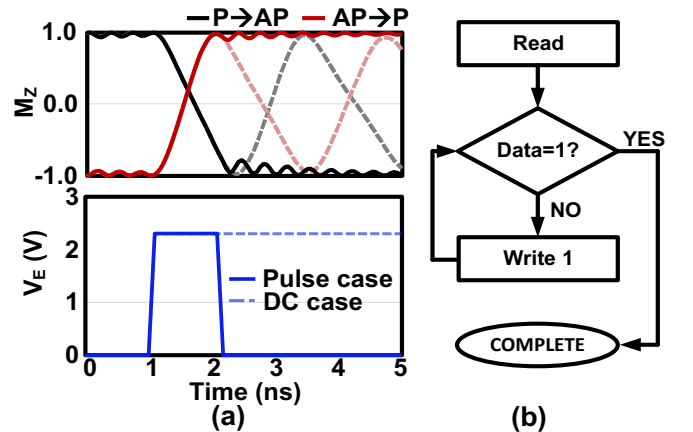
Fig. 4. VCMA only switching scheme: (a) Write voltage ( V_{MTJ} ) pulse and magnetization switching simulation results for VCMA device; (b) Flowchart for writing "1" into a VCMA MTJ. Due to the inherent non-deterministic switching of VCMA, a read operation is required before each write operation.
