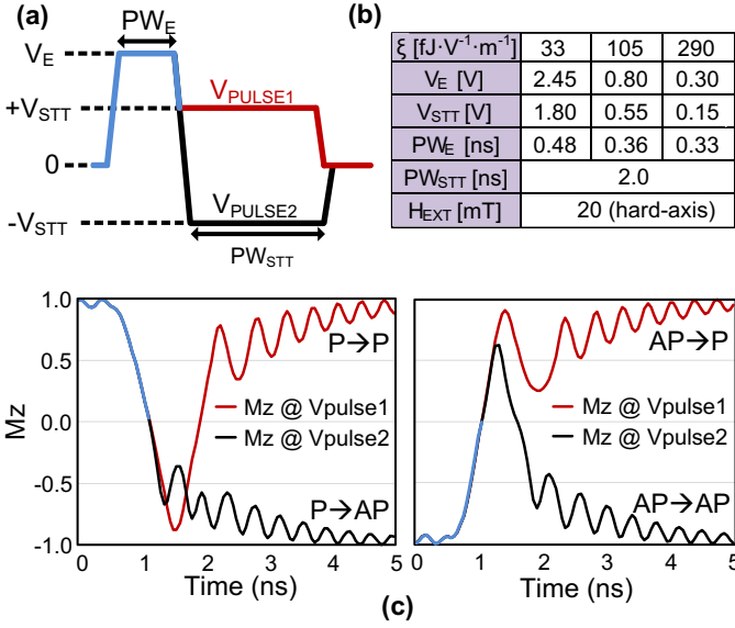
Fig. 5. VCMA-assisted STT switching scheme: (a) V_{MTI} waveform where an initial high voltage is followed by a positive or negative STT pulse; (b) simulation parameters; (c) magnetization dynamics for P→P, P→AP, AP→P, and AP→AP switching.
