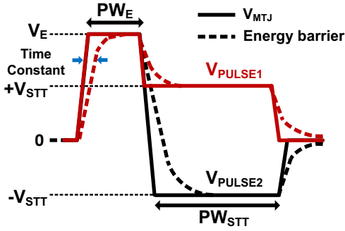
Fig. 8. Concept of time constant between applied voltage and energy barrier.
