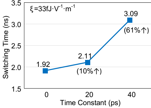
Fig. 9. Effect of energy barrier time constant on switching time.
