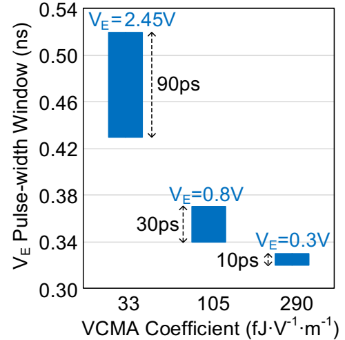
Fig. 7. Pulse width window for different VCMA coefficients.
