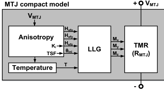
Fig. 3. Proposed VCMA based MTJ SPICE compact model.
