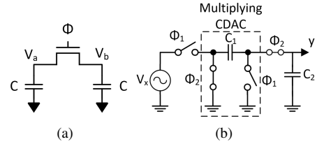
Figure 3: Implementation of addition operation (a) circuit diagram of addition operation using charge sharing [12], and (b) circuit diagram of multiplying passive analog MAC implementations [17].
