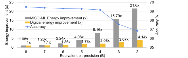
Figure 6: MiSO-ML energy vs. accuracy trade-off plot for different noise threshold constraints for the ResNet18 architecture using an ImageNet workload. MiSO-ML energy improvement (gray columns) is nonlinear while digital energy improvement is modest (yellow bars).
