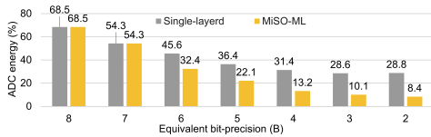
Figure 7: ADC energy (% of total energy) vs. noise threshold constraints for ResNet18. Gray bars: ADC inserted after each layer [9].
