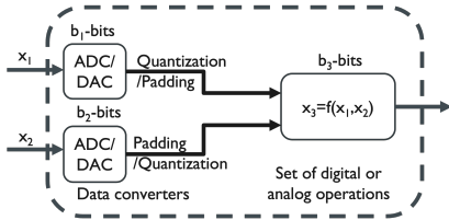
Figure 1: Building block diagram of the MiSO-ML unit.
