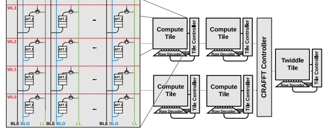
Fig. 5. CRAFFT organization.
