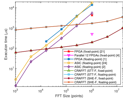
Fig. 6. Fixed-point and floating point execution times vs. various baselines.
