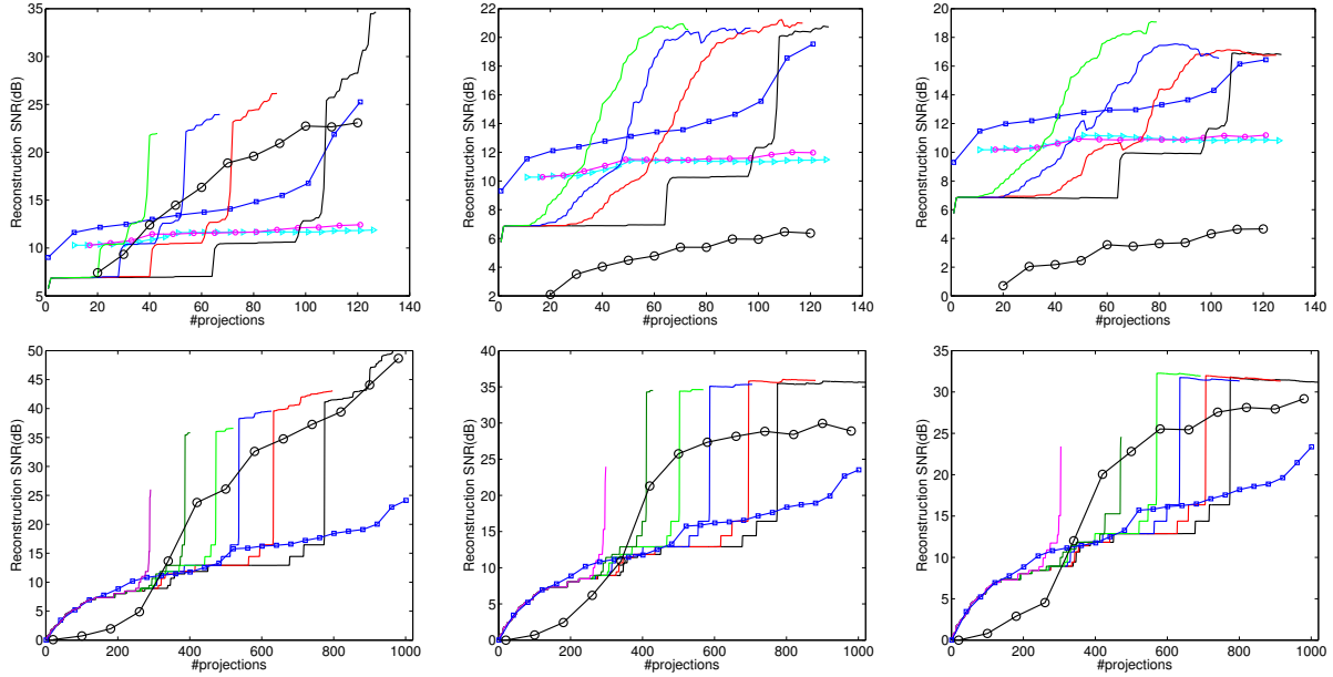
Fig. 2: SNR vs. Number of measurements plots (best viewed in color) with different noise levels and for different schemes (LAsER, PCA, direct wavelet sensing, and CS/LASSO). The top row corresponds to reconstruction SNR achieved when acquiring a test image from the PICS database (column 1: \sigma = 0 , column 2: \sigma = 0.3 , column 3: \sigma = 0.8 ). Here, \square is PCA, black \circ is LASSO, sky blue \triangleright and magenta \circ are for direct wavelet sensing with \tau = 0 and \tau = 0.5 respectively. Colored solid lines (left to right) are for LAsER with \tau = 0, 0.3, 0.5 , and 2. The bottom row corresponds to reconstruction SNR achieved when acquiring a test image from the synthetically generated data (column 1: \sigma = 0 , column 2: \sigma = 3 , column 3: \sigma = 5 ). Here, \square is PCA, \circ is CS/LASSO. Colored solid lines (left to right) are for LAsER with \tau = 0, 1, 2, 3, 5 and 8 respectively.
